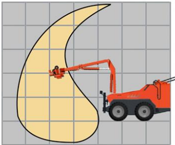
Horizontal drilling, sideways
