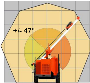
Horizontal drilling, sideways With manual roll-over
