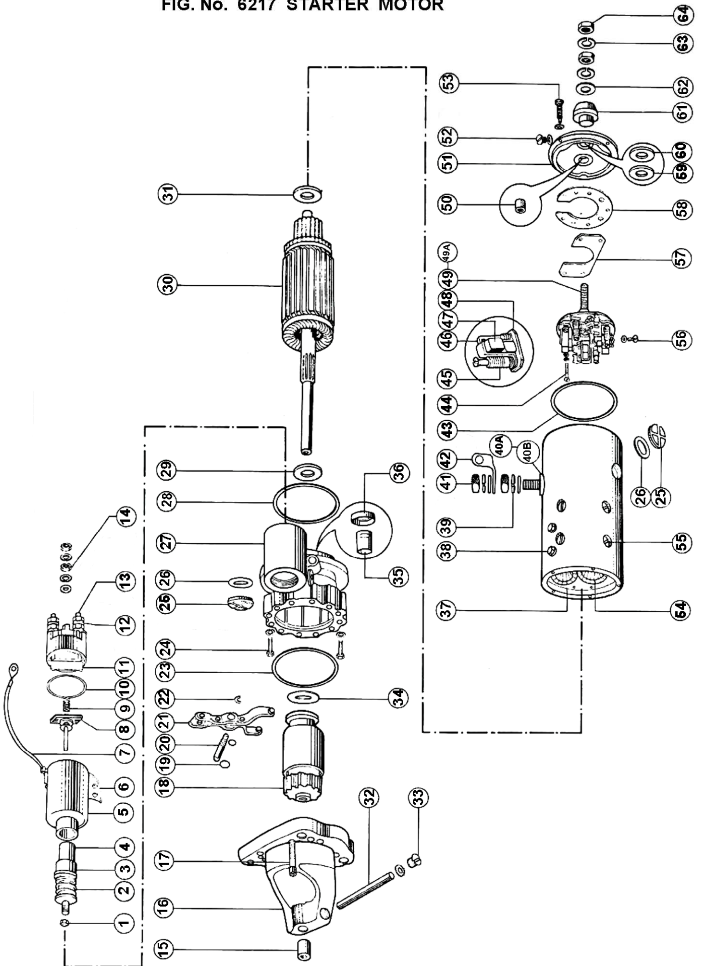
FIG. No. 6217 STARTER MOTOR
